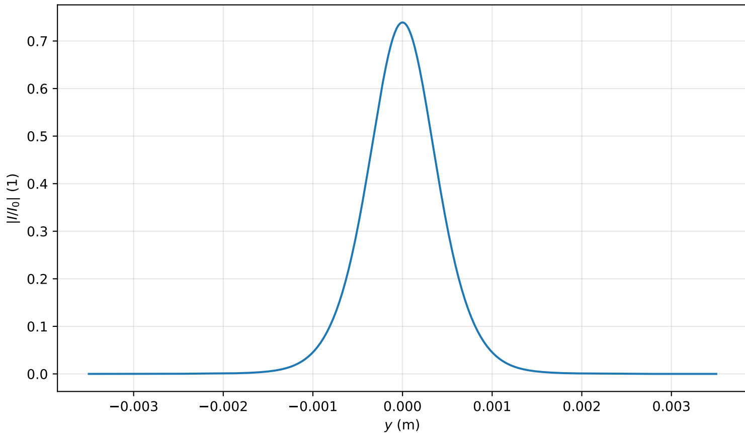
Intensity profile I(x=0, y, z=3.423)/I_0 , P_{in}=0.7P_{cr} , artificial time
